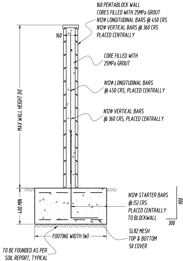
TYPICAL 160 WIDE PENTABLOCK FENCE WALL NTS
